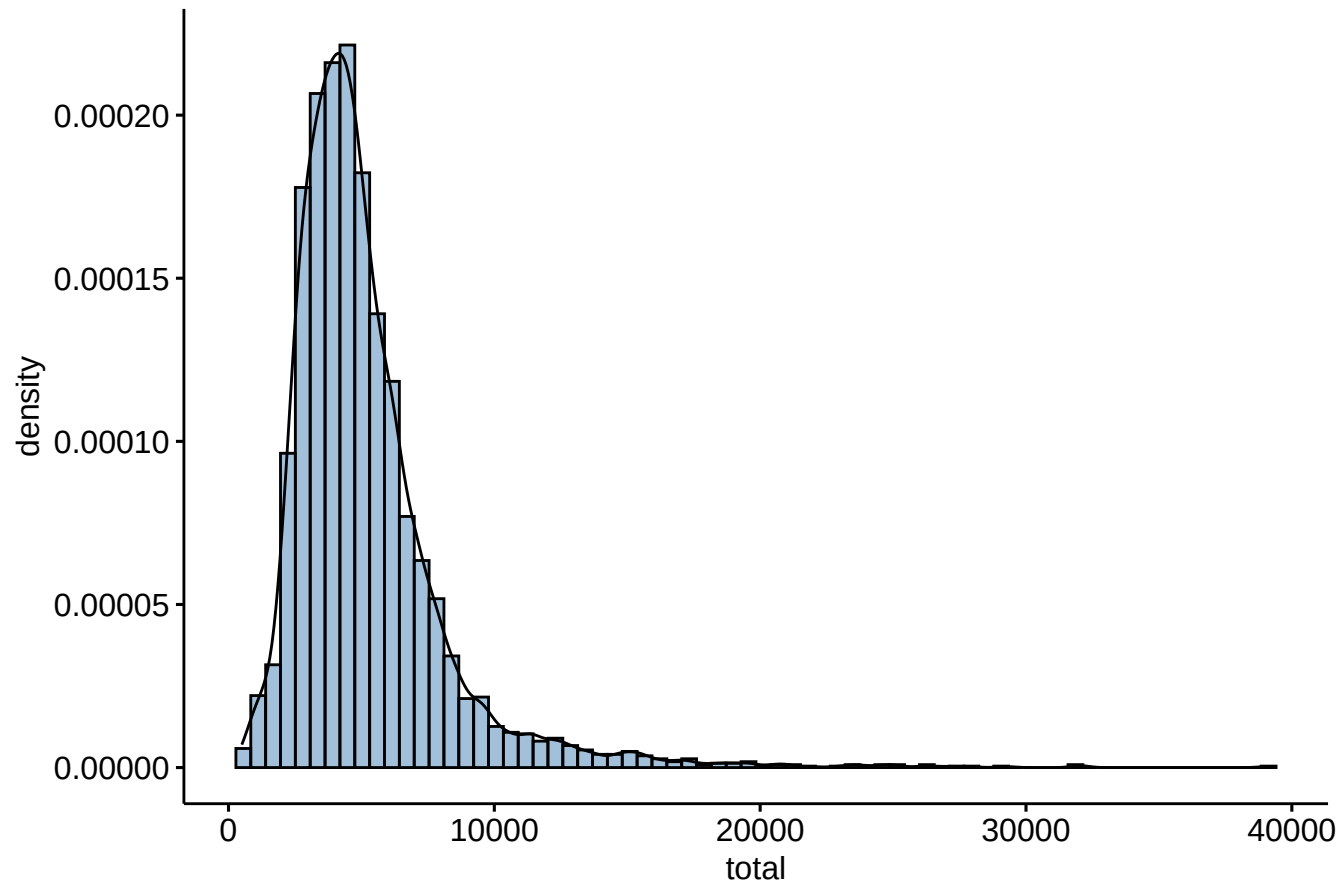
Cluster 8
